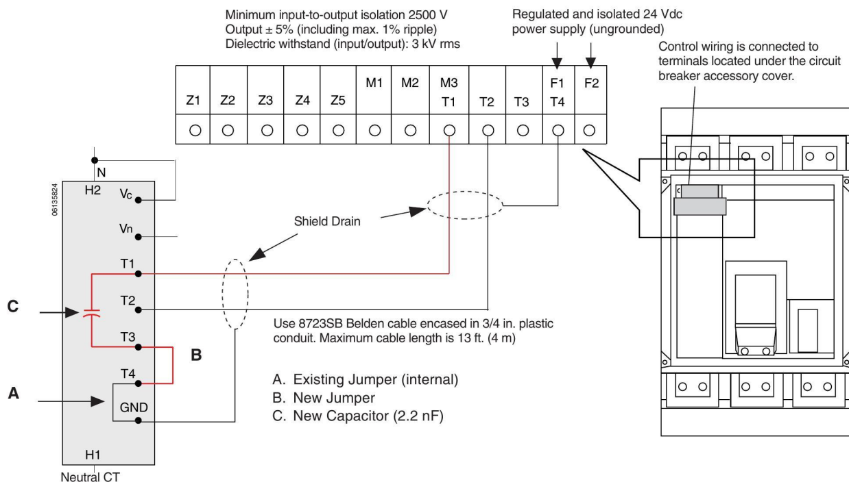
Figure 17: Wiring Schematic
